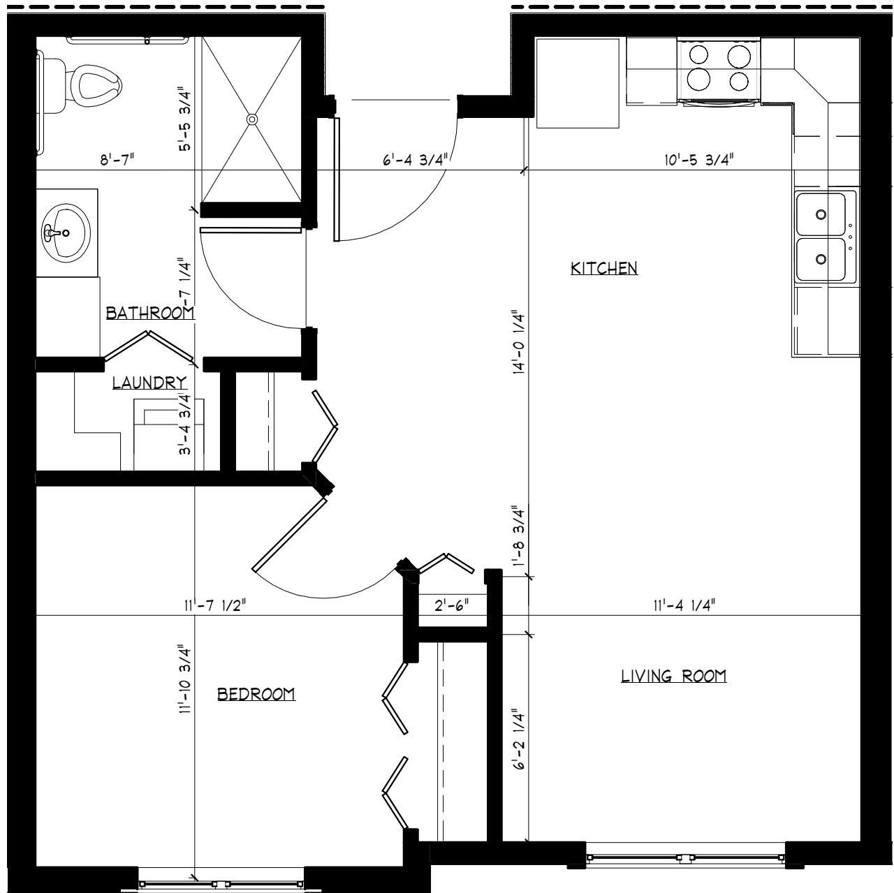
1 UNIT B1 PLAN - 583 SF SCALE: 1/4" = 1'-0" $2,689.00
