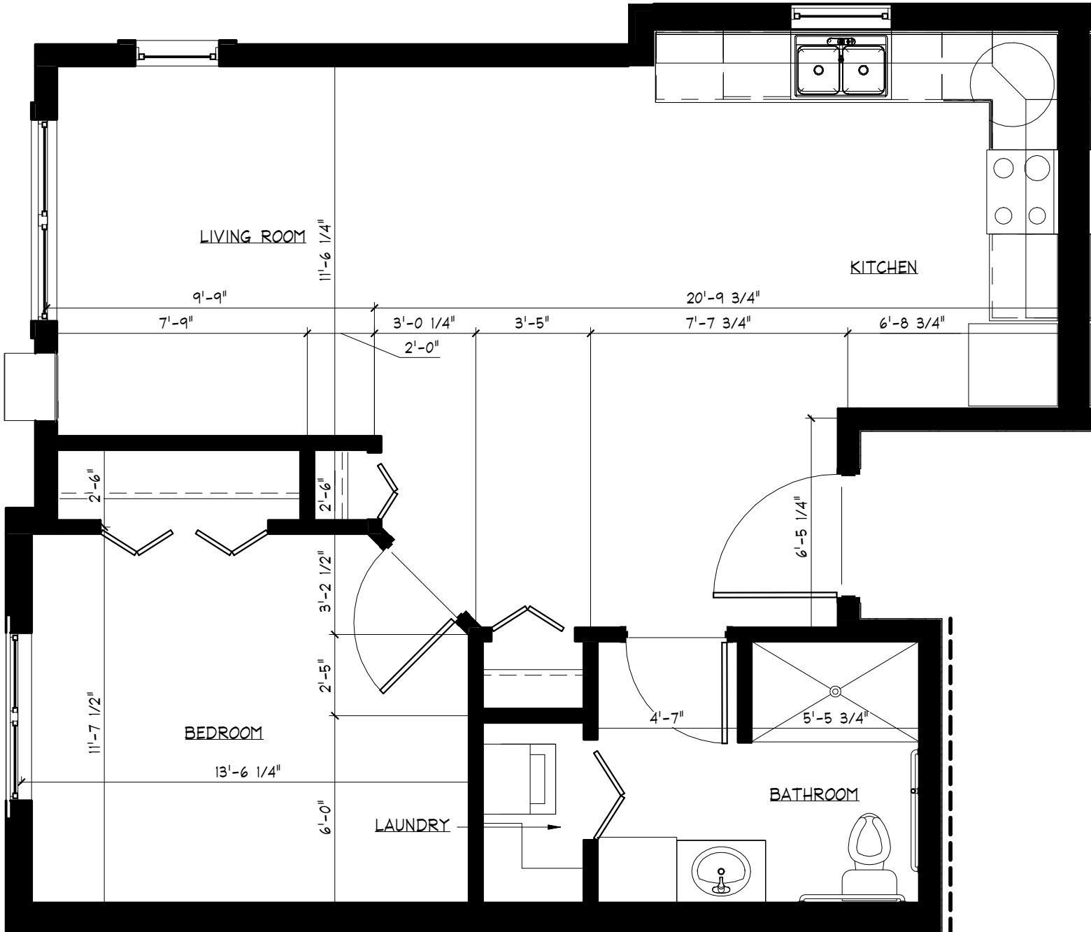
1 UNIT A2 PLAN - 686 SF SCALE: 1/4" = 1'-0" $3,162.00
