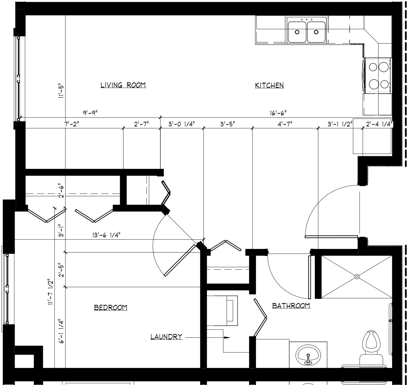
1 UNIT B2 PLAN - 619 SF SCALE: 1/4" = 1'-0" $2,854.00
